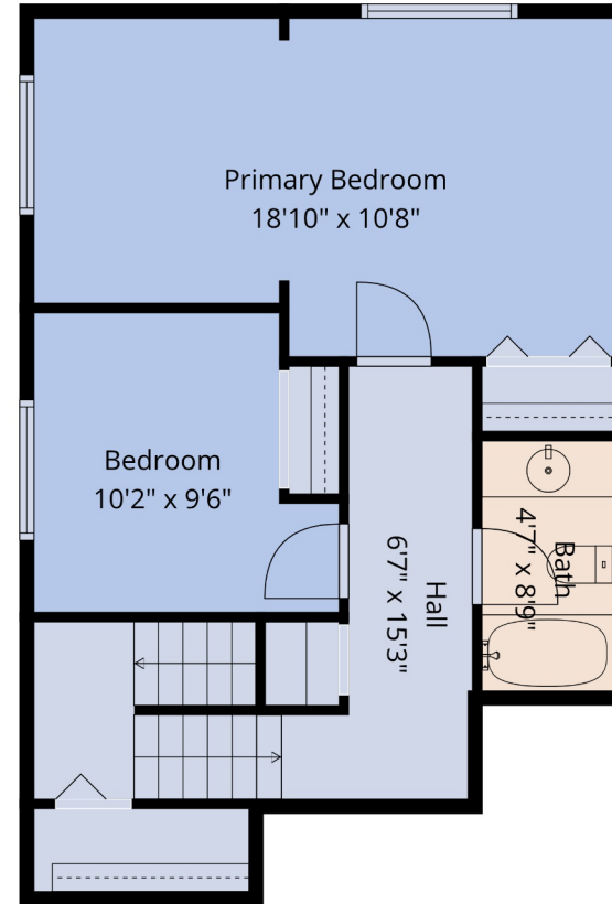
2nd Floor
