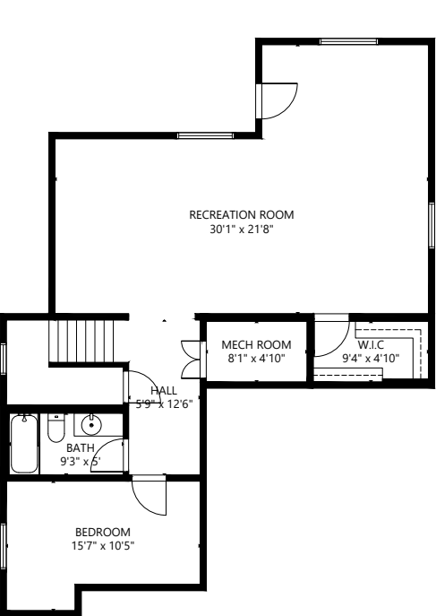
BASEMENT 1083 SQ. FT.
