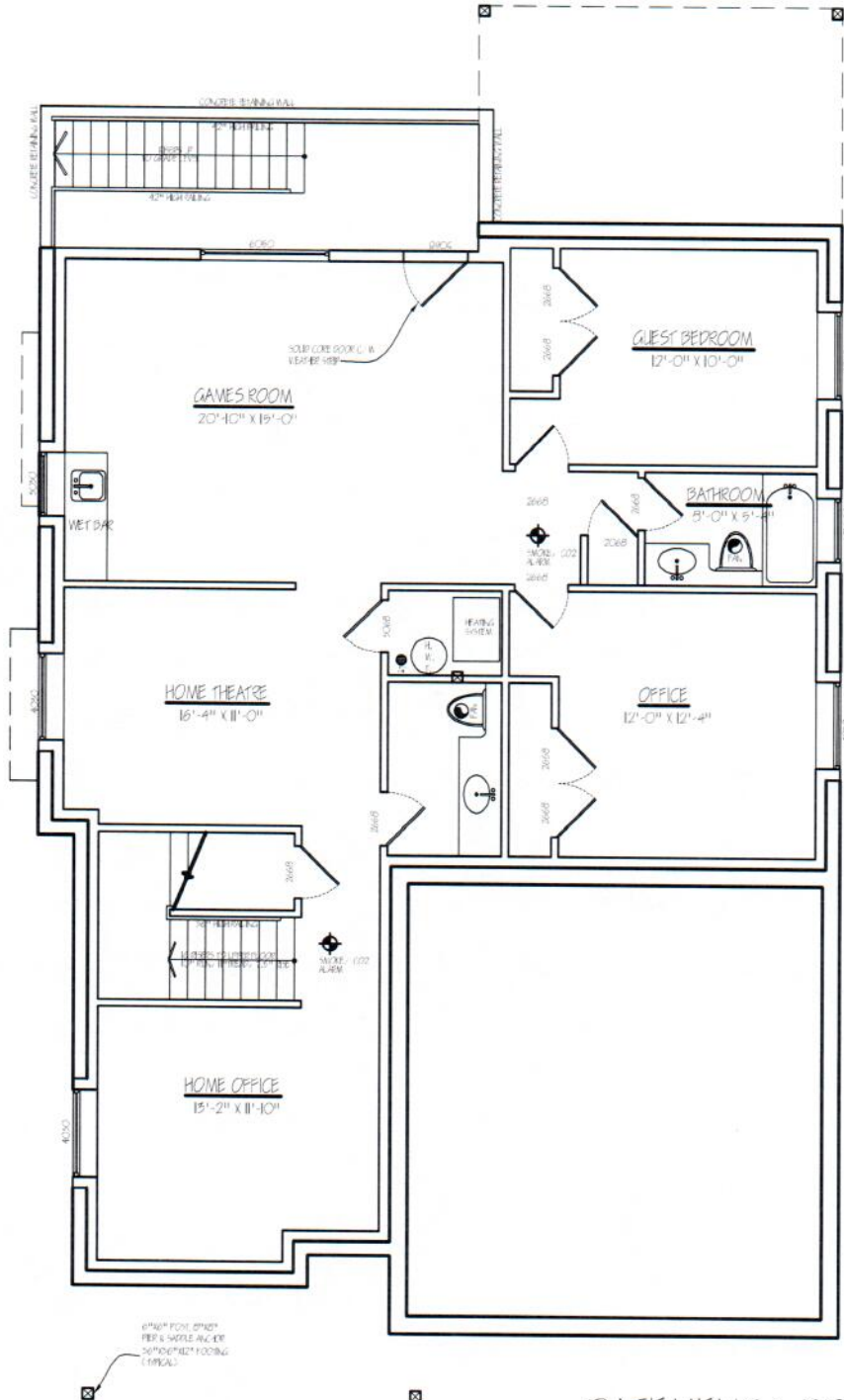
BASEMENT & FOUNDATION PLAN FLOOR AREA: 1,592 sq.ft.
