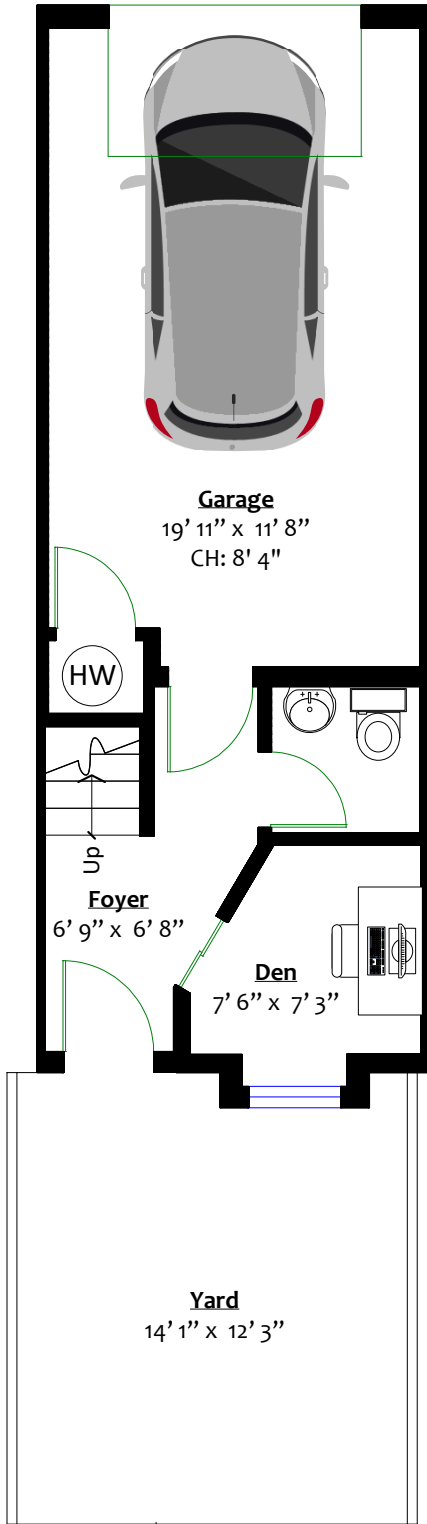
LOWER LEVEL Floor Area: 157 Sq. Ft. Ceiling Height: 8'
