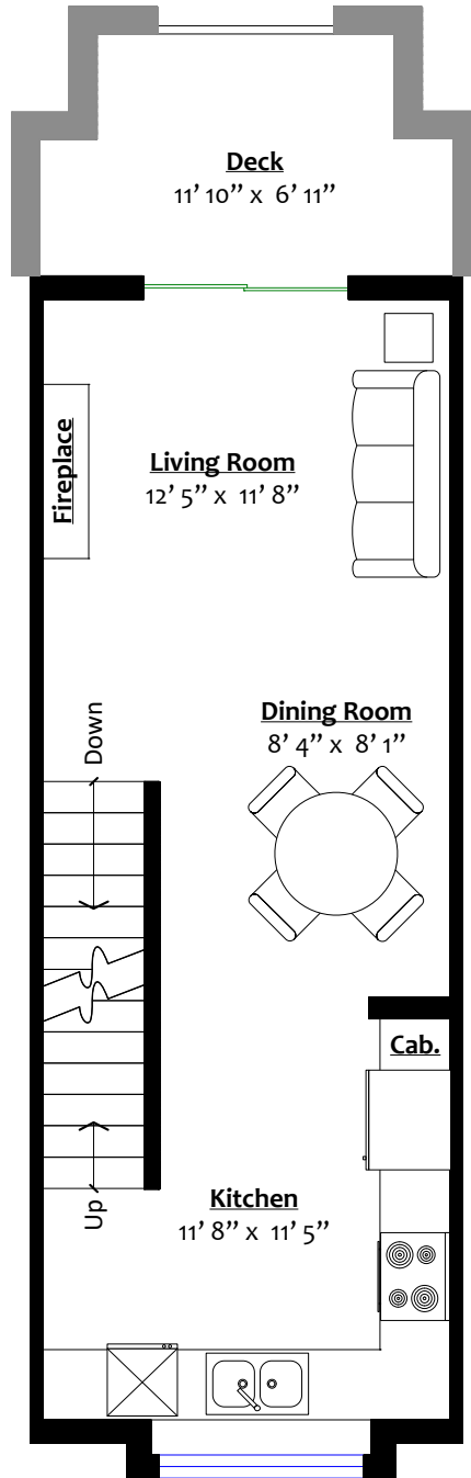
MAIN LEVEL Floor Area: 409 Sq. Ft. Ceiling Height: 9'
