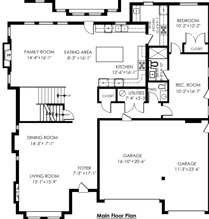
Main Floor Plan Floor Area: 1906 sq.ft. Ceiling Height: 10'
