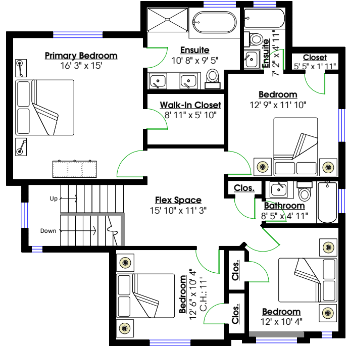
UPPER LEVEL Floor Area: 1,284 Sq. Ft. Ceiling Height: 9'
