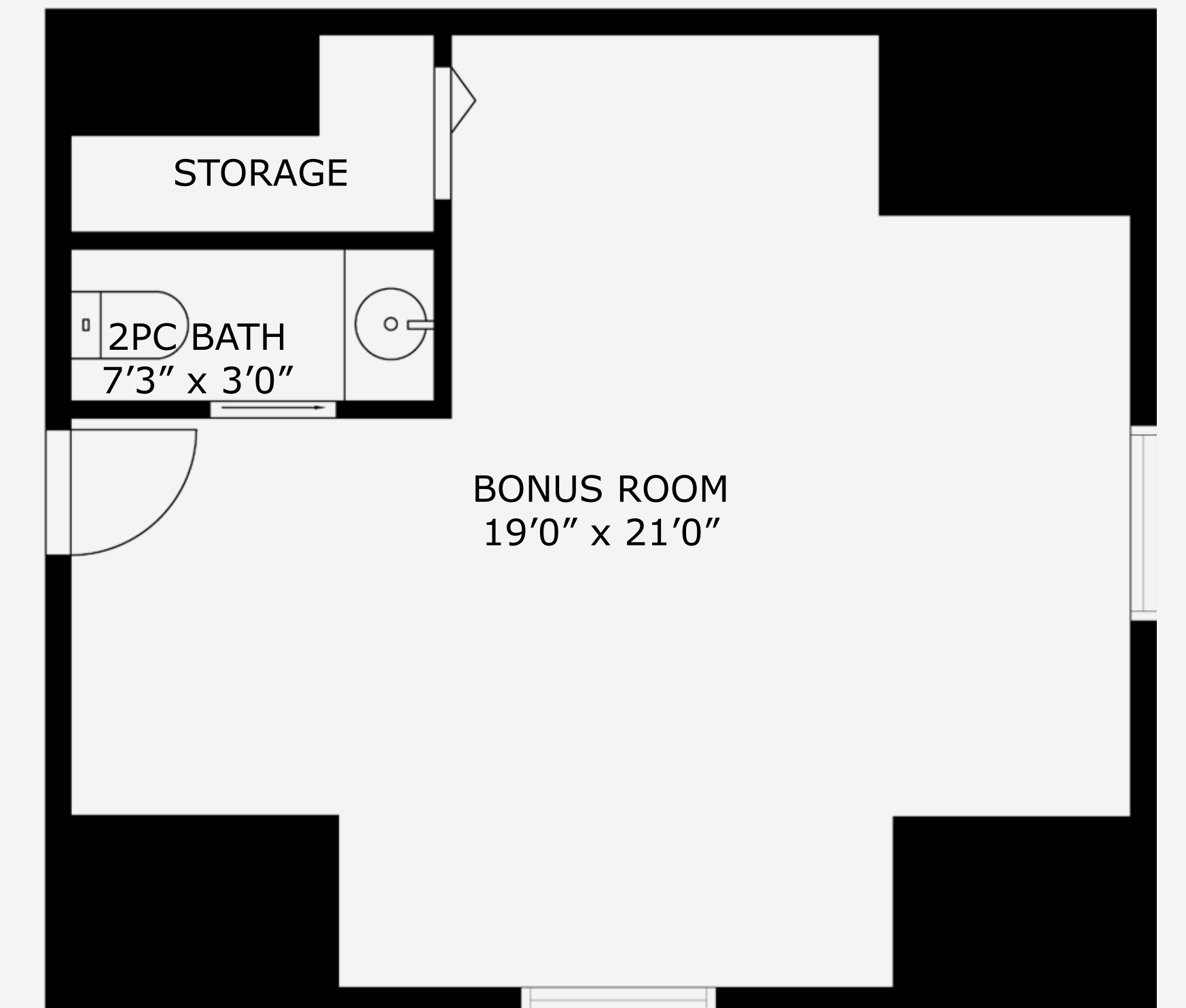
SUITE ABOVE GARAGE (380 sq/f) VAULTED CEILING - 9'0"
