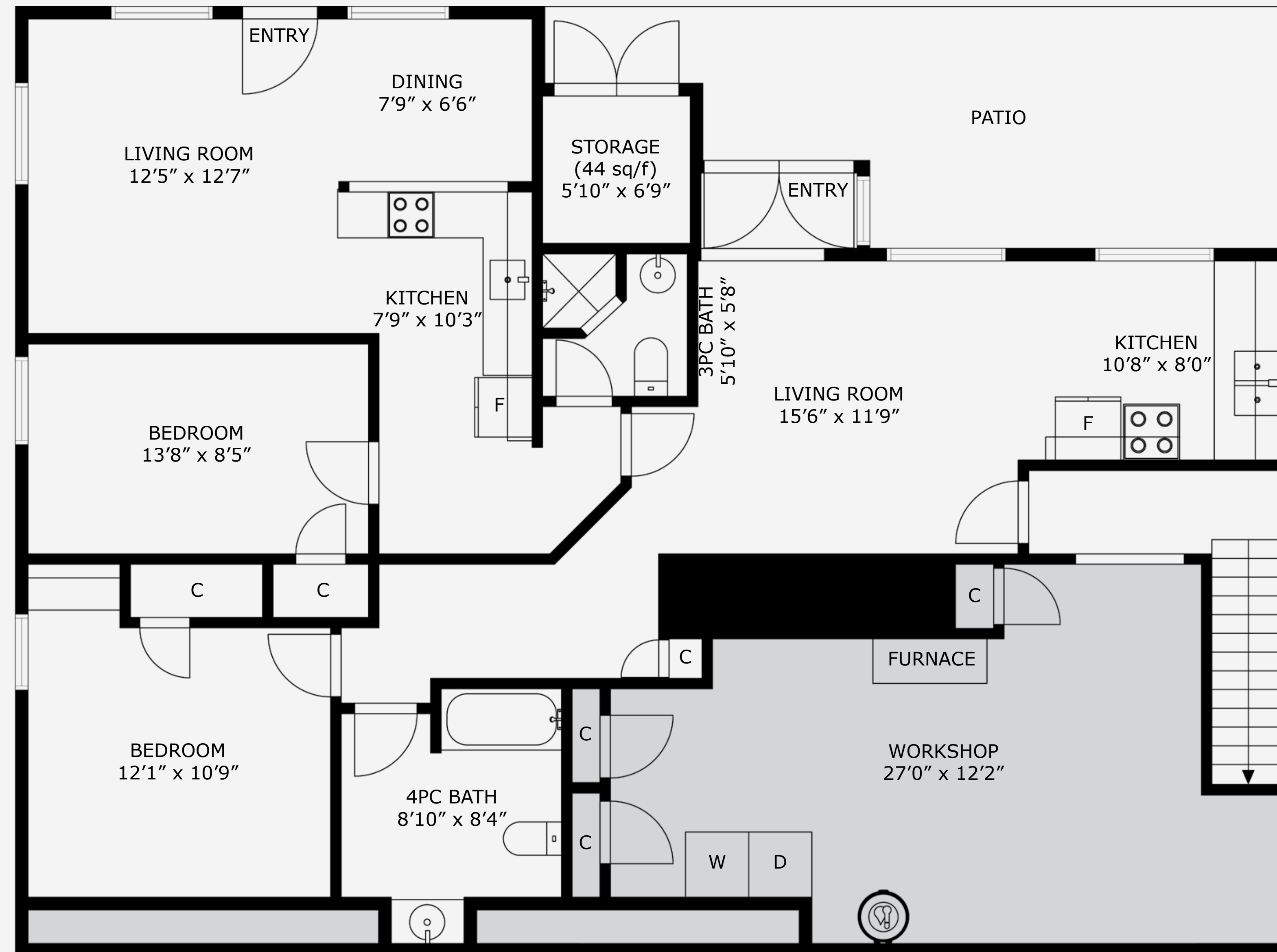
LOWER LEVEL (FINISHED - 1244 sq/f, UNFINISHED - 432 sq/f) CEILING HEIGHT - 7'2"
