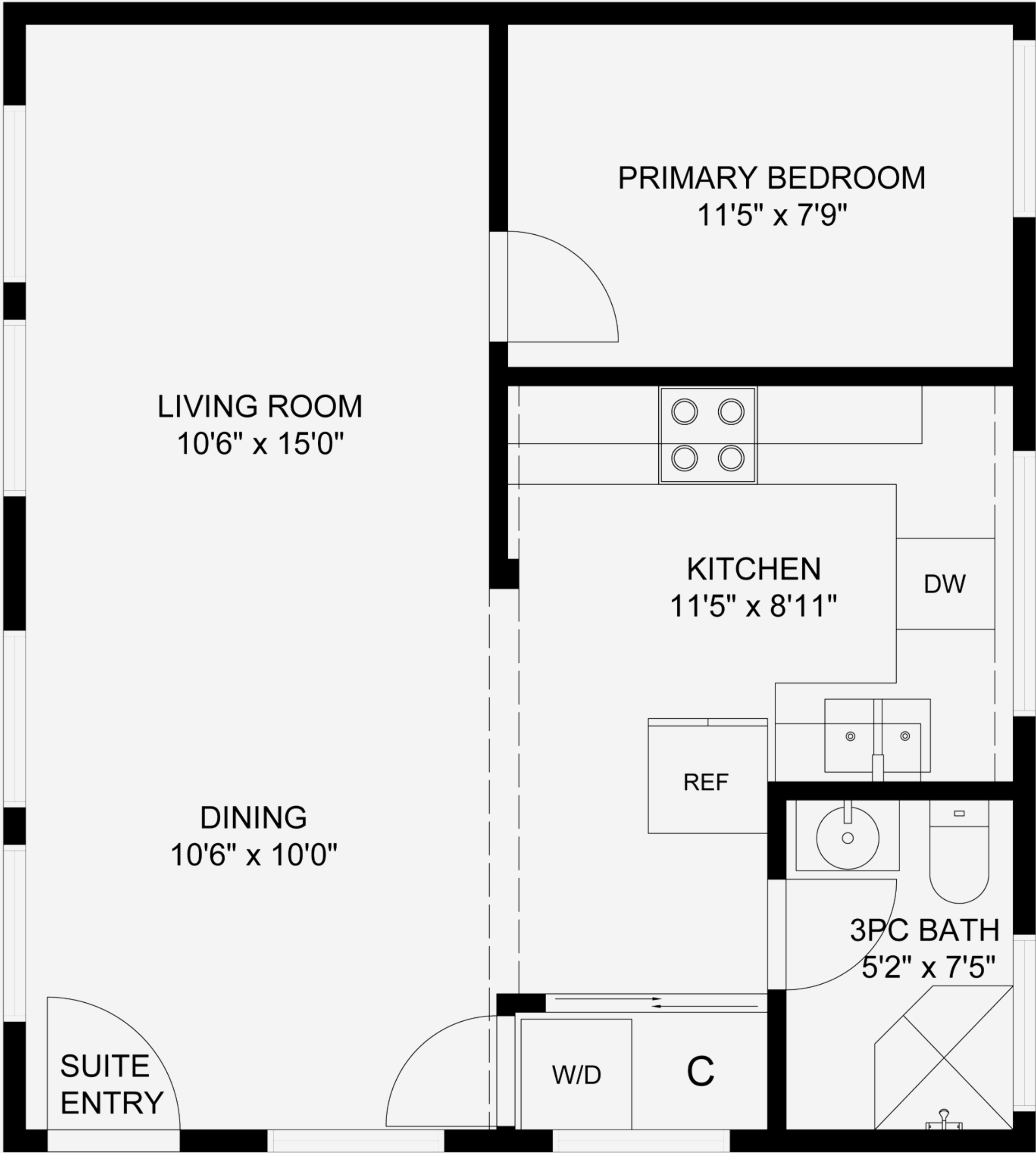
MAIN LEVEL - 606 SQFT CEILING HEIGHT - 9'6"
