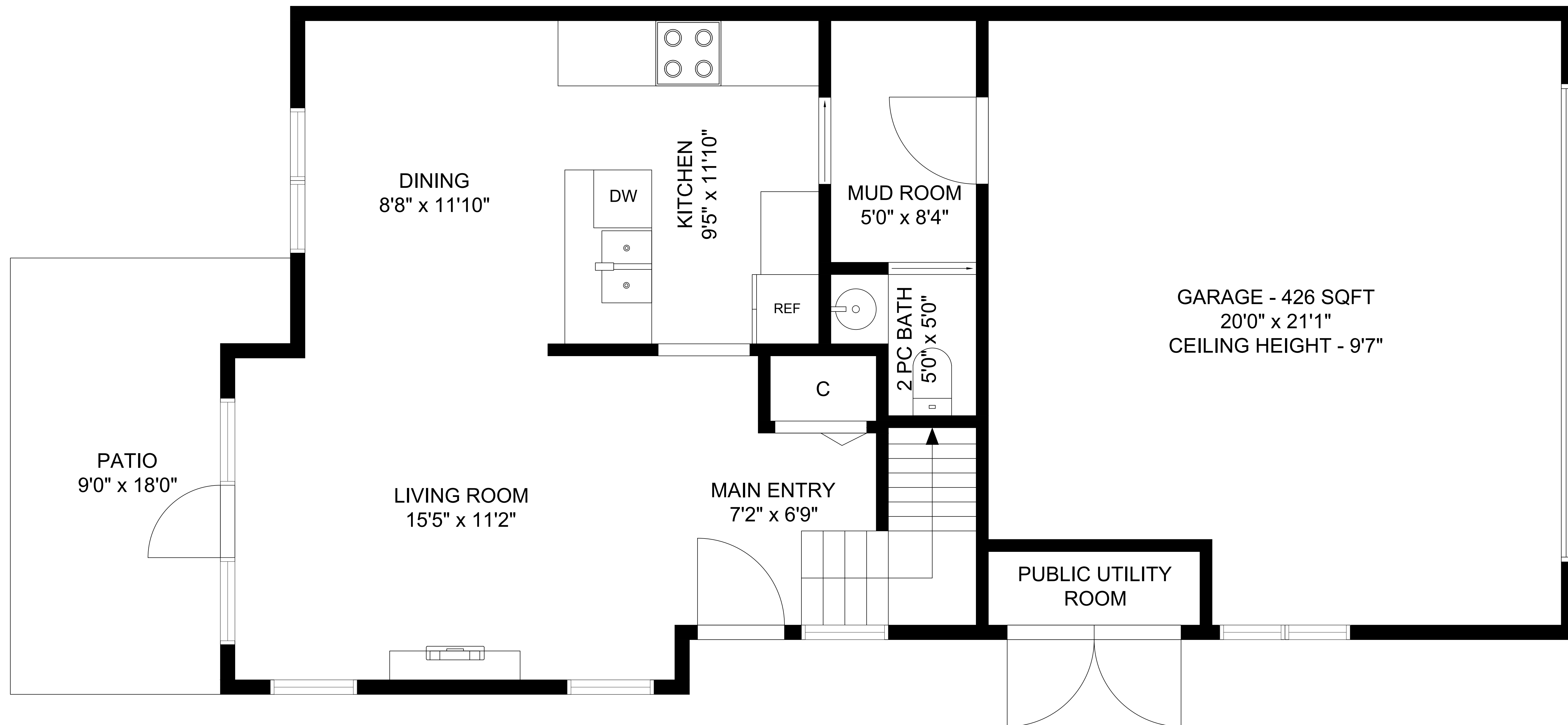
MAIN LEVEL - 566 SQFT CEILING HEIGHT - 9'0"
