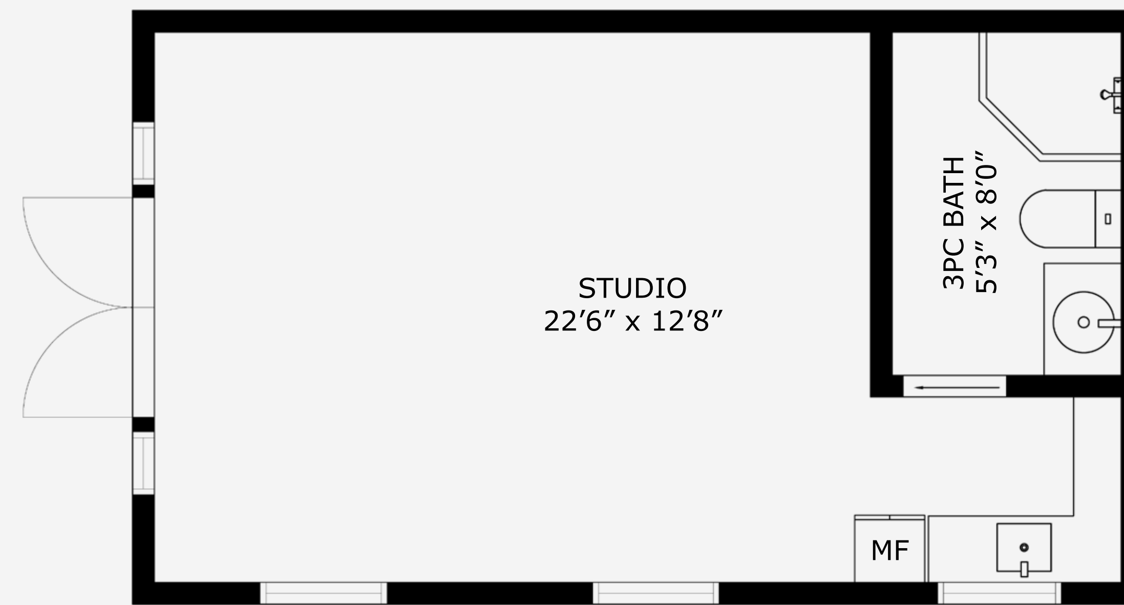
STUDIO (322 sq/f) CEILING HEIGHT - 8'0"
