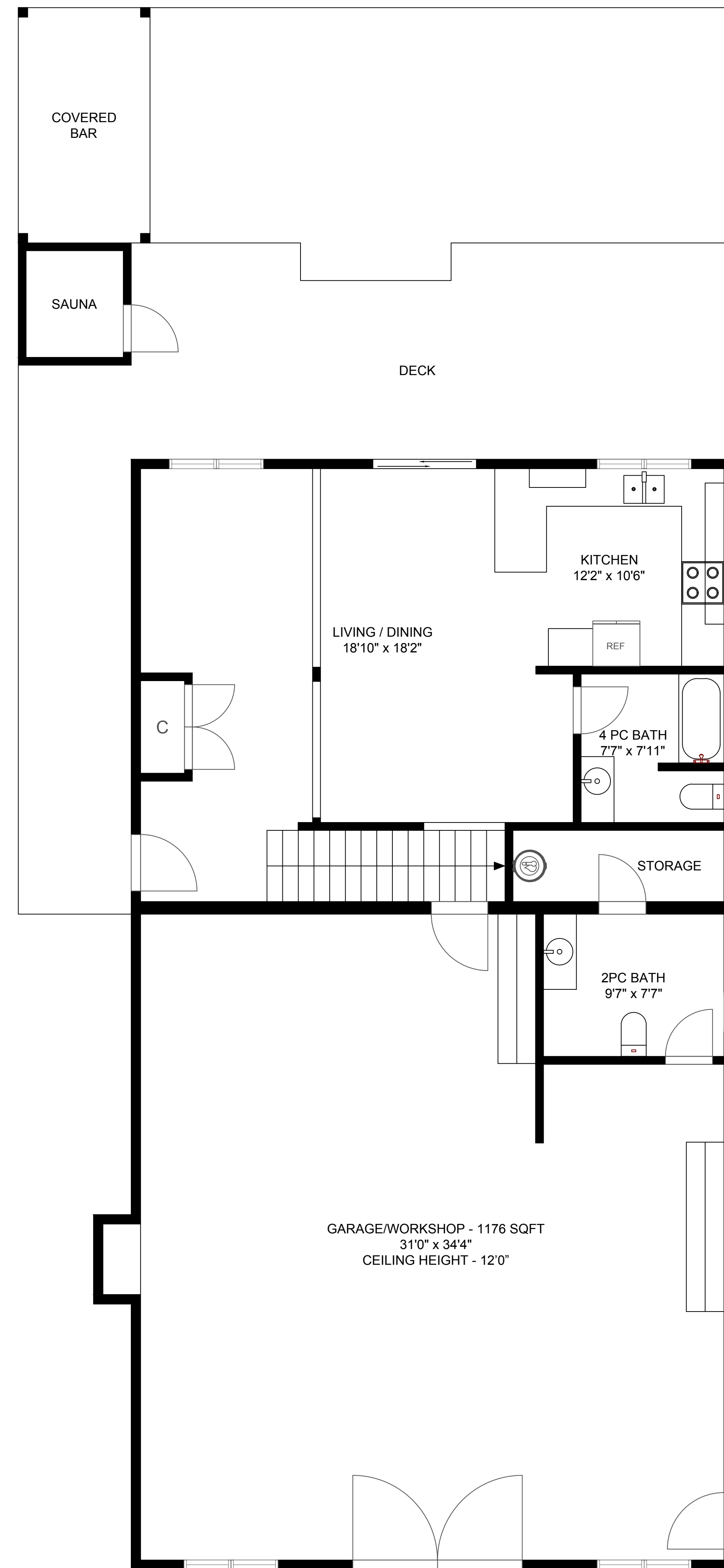
SECONDARY RESIDENCE MAIN LEVEL - 722 SQFT CEILING HEIGHT - 9'0"
