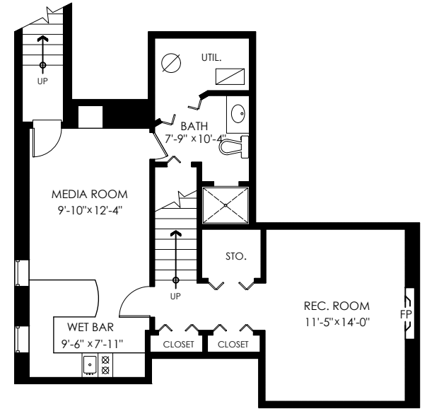
Lower Floor Plan Floor Area: 675 sq.ft. Ceiling Height: 7'-3"
