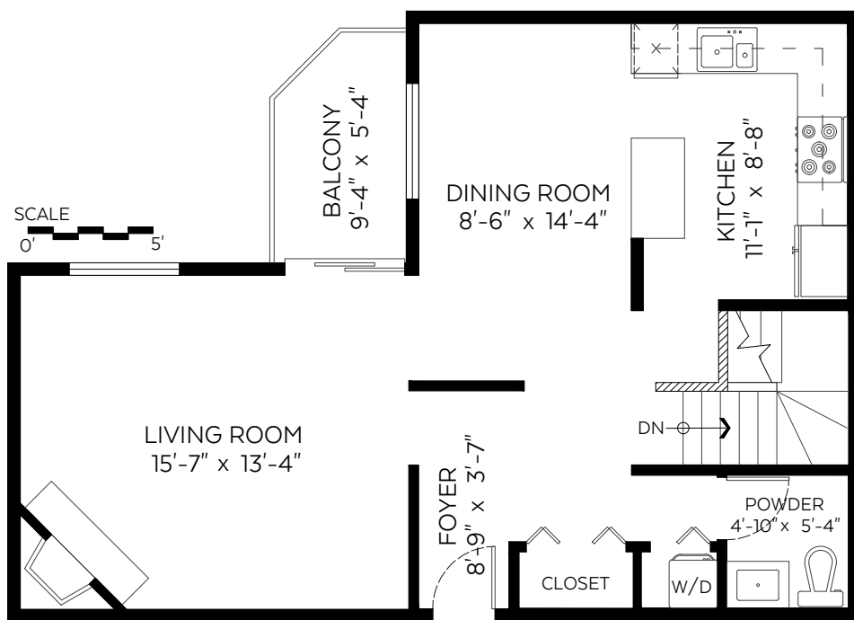
Main Floor Plan Floor Area: 674 sq.ft.
