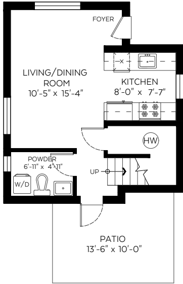
Laneway Main Floor Plan Floor Area: 410 sq.ft. Ceiling Height: 8 ft.
