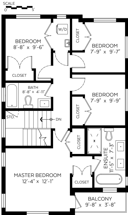
Upper Floor Plan Floor Area: 872 sq.ft. Ceiling Height: 9 ft.
