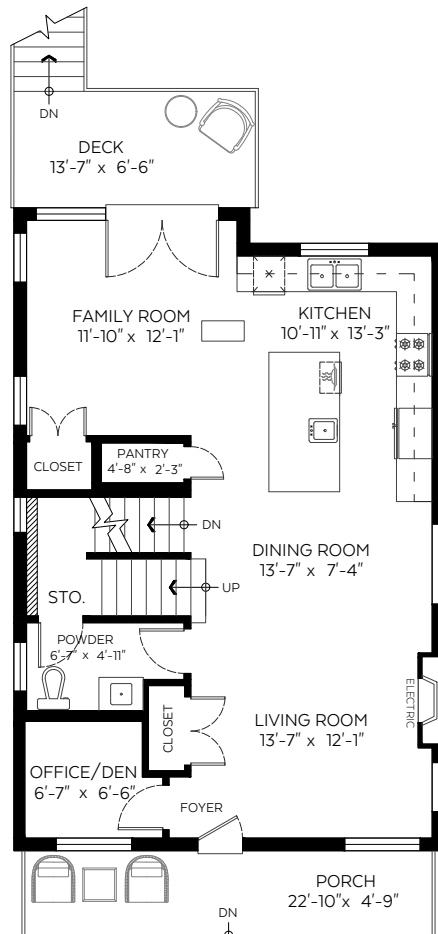
Main Floor Plan Floor Area: 851 sq.ft. Ceiling Height: 10 ft.
