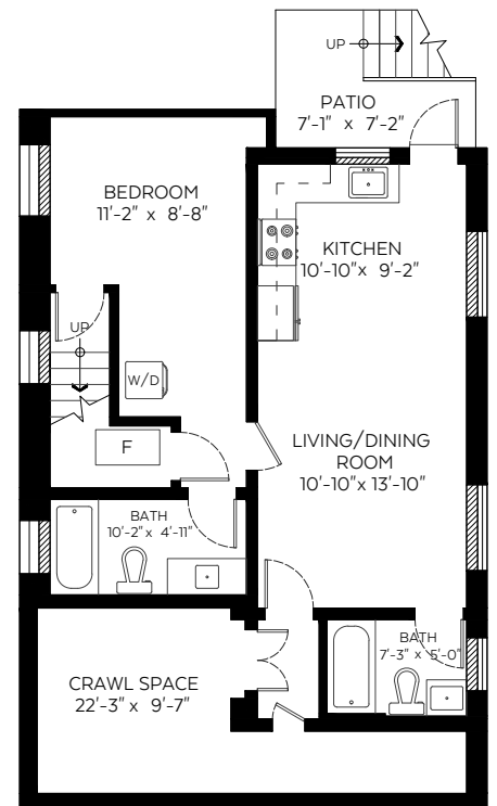
Lower Floor Plan Floor Area: 684 sq.ft. Ceiling Height: 8 ft.
