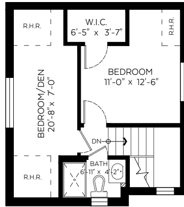
Laneway Upper Floor Plan Floor Area: 438 sq.ft. Ceiling Height: 8.75 ft.
