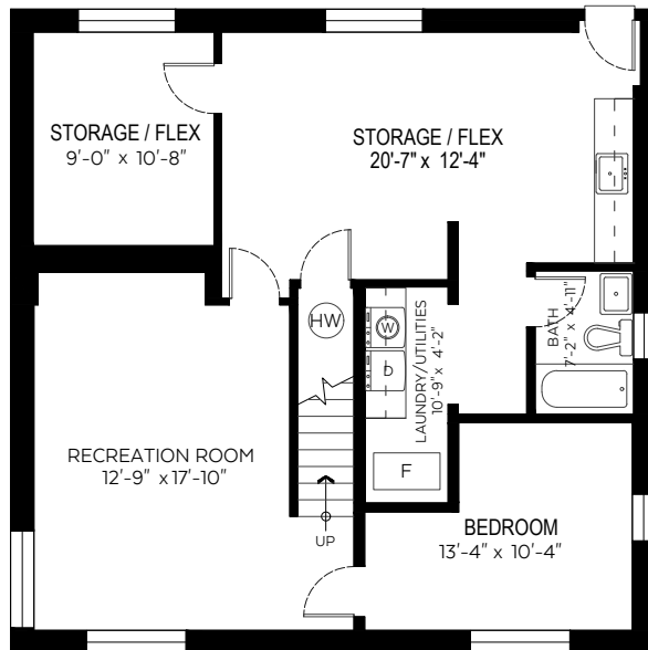
Lower Floor Plan Floor Area: 1,033 sq.ft.
