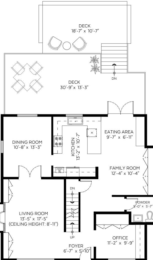
Main Floor Plan Floor Area: 1,070 sq.ft.
