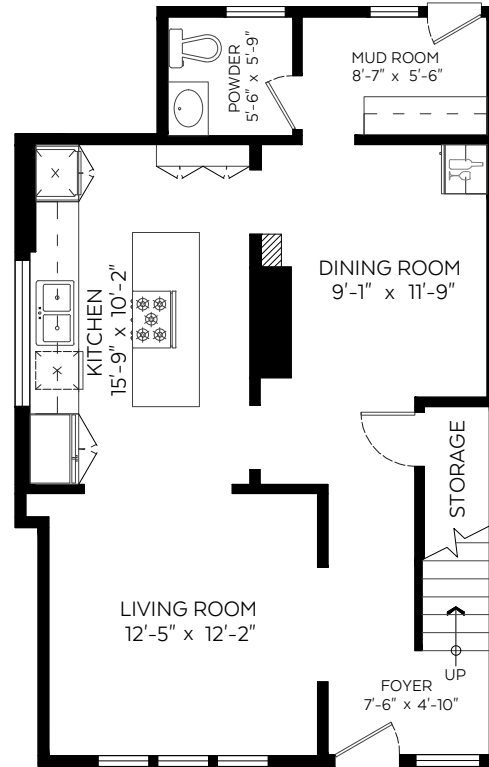
Main Floor Plan Floor Area: 741 sq.ft.
