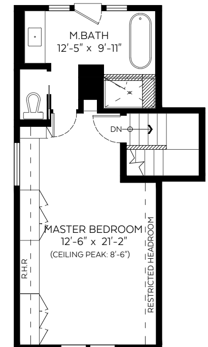
Top Floor Plan Floor Area: 397 sq.ft.
