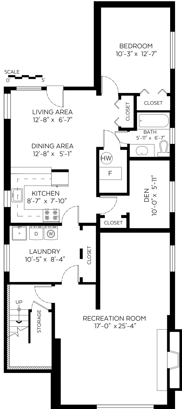
Lower Floor Plan Floor Area: 1,310 sq.ft.
