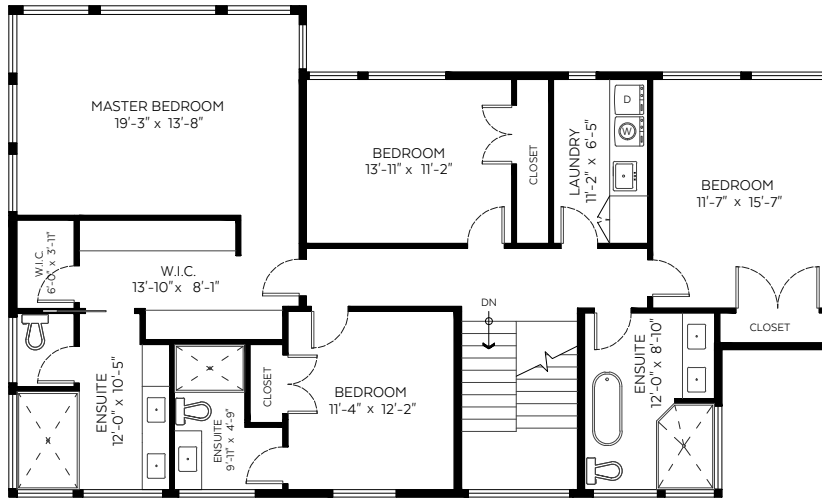
Upper Floor Plan Floor Area: 1,632 sq.ft. Ceiling Height: 9 ft.
