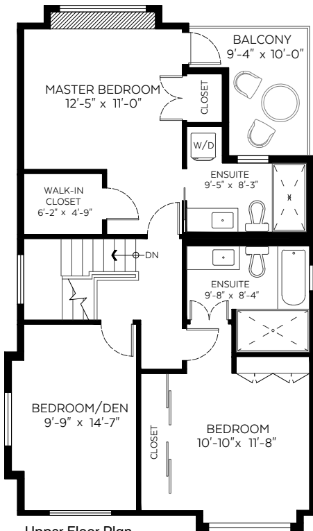
Upper Floor Plan Floor Area: 839 sq.ft. Ceiling Height: 9 ft.
