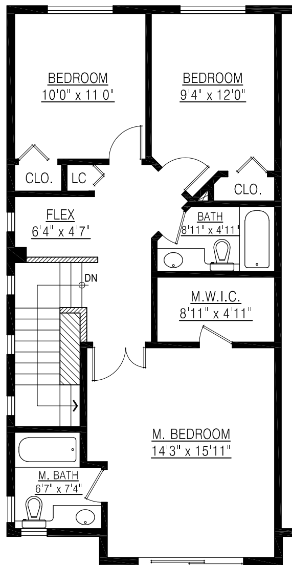
UPPER FLOOR PLAN FLOOR AREA: 834 sq.ft.
