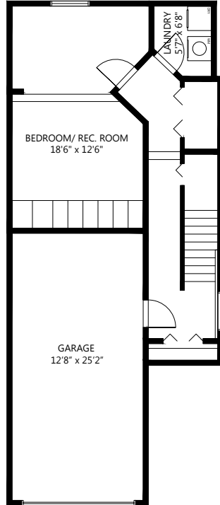
Lower Level: 562 SQ.FT. Ceiling Height: 8'0"
