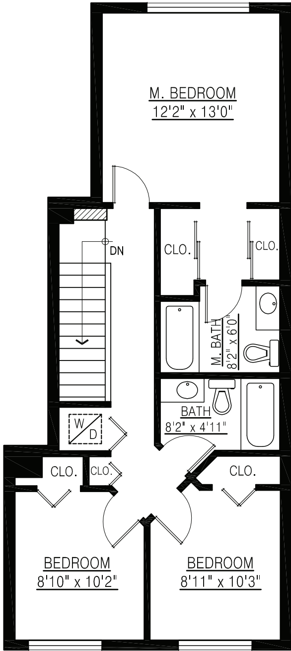
UPPER FLOOR PLAN FLOOR AREA: 691 sq.ft.
