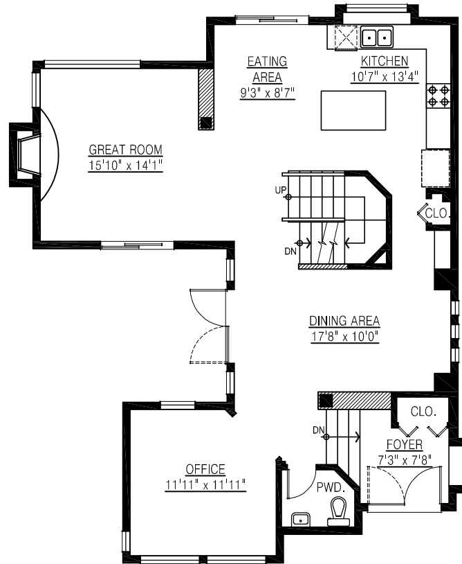
MAIN FLOOR PLAN FLOOR AREA: 1,147 sq.ft.
