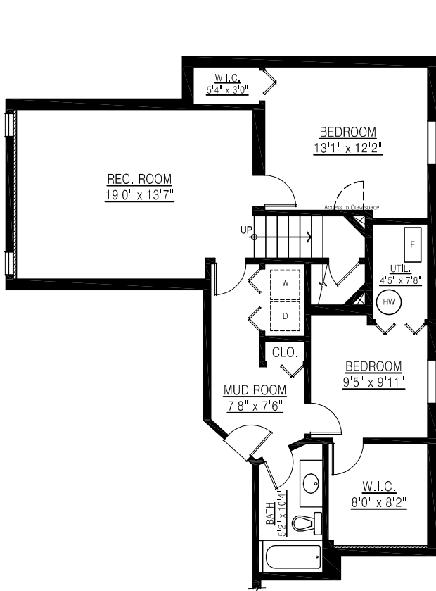
BASEMENT FLOOR PLAN FLOOR AREA: 978 sq.ft.
