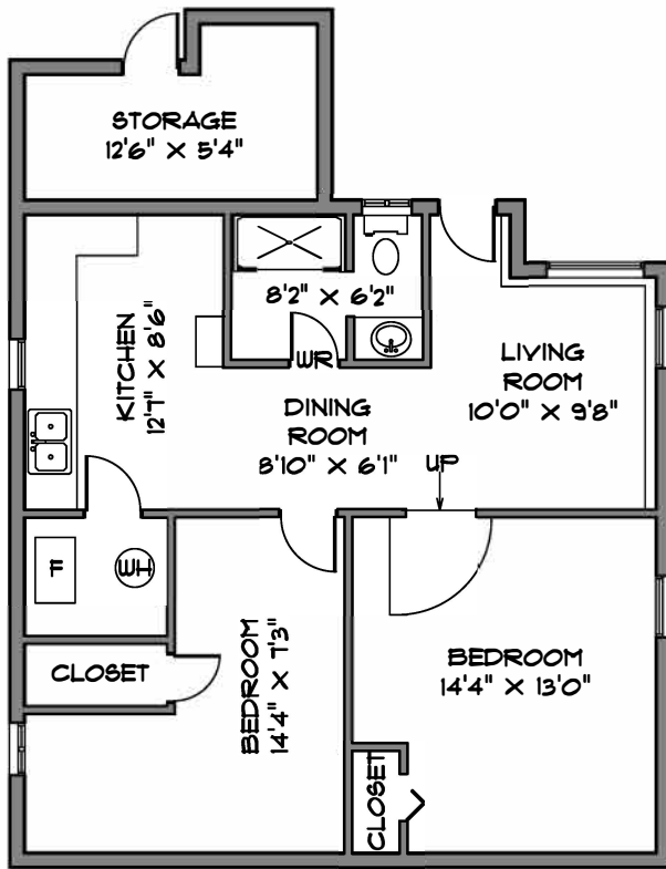
LOWER LEVEL 894 SQ. FT.
