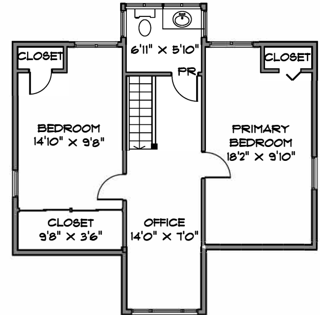
UPPER LEVEL 618 SQ. FT.
