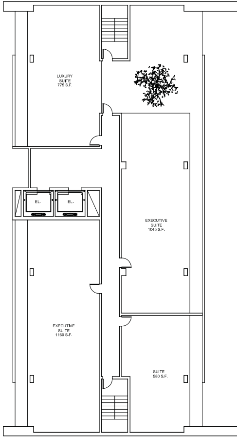
TYPICAL FLOOR – EXECUTIVE SUITES x1 SCALE: 1:100
