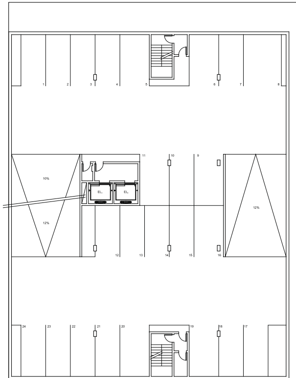
PARKING LEVEL 1 SCALE: 1:100
