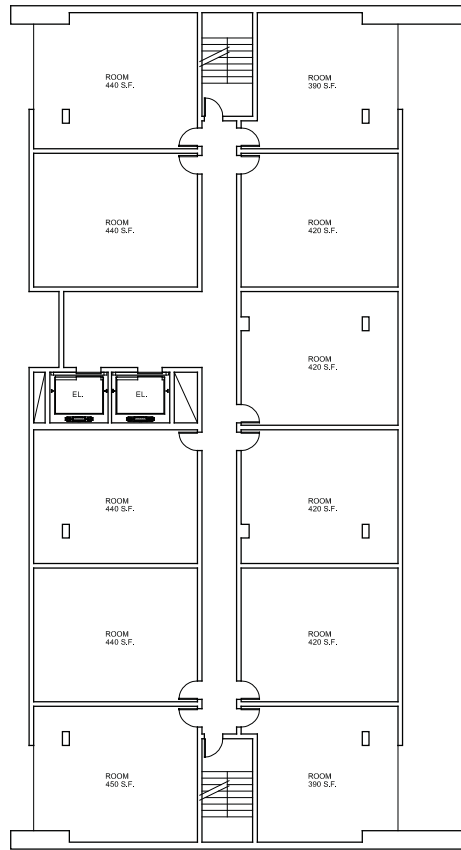
TYPICAL FLOOR – ROOMS x6 SCALE: 1:100
