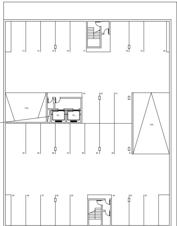
PARKING LEVEL 4 SCALE: 1:100
