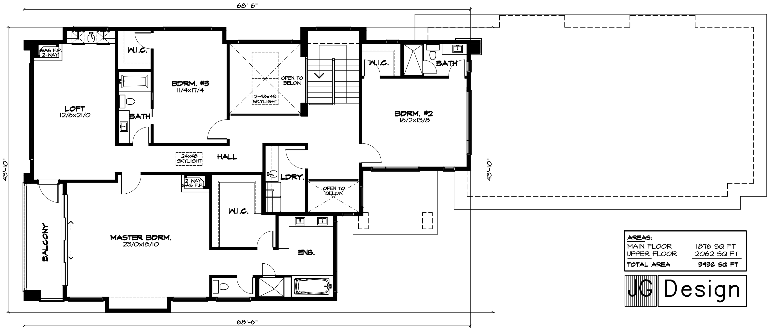
UPPER FLOOR PLAN
