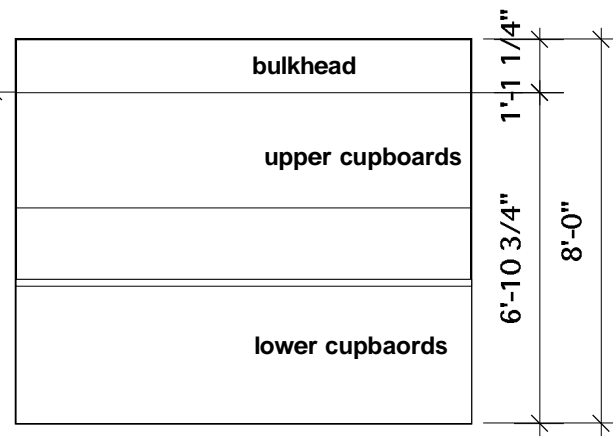
2 kitchen elevation Scale: 1/4" = 1'-0"
