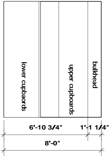
2 Kitchen elevation Scale: 1/4" = 1'-0"
