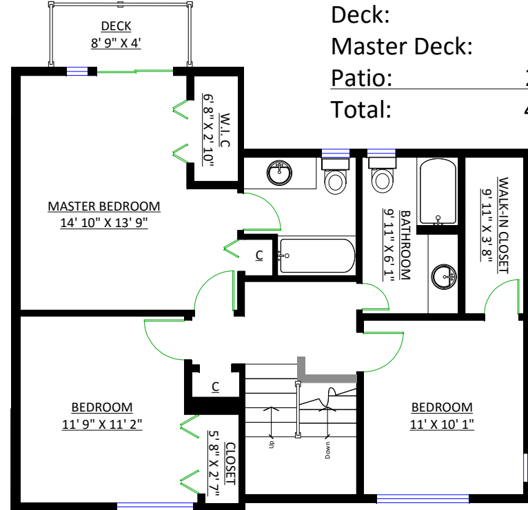
UPPER LEVEL Floor Area: 811 Sq. Ft.
