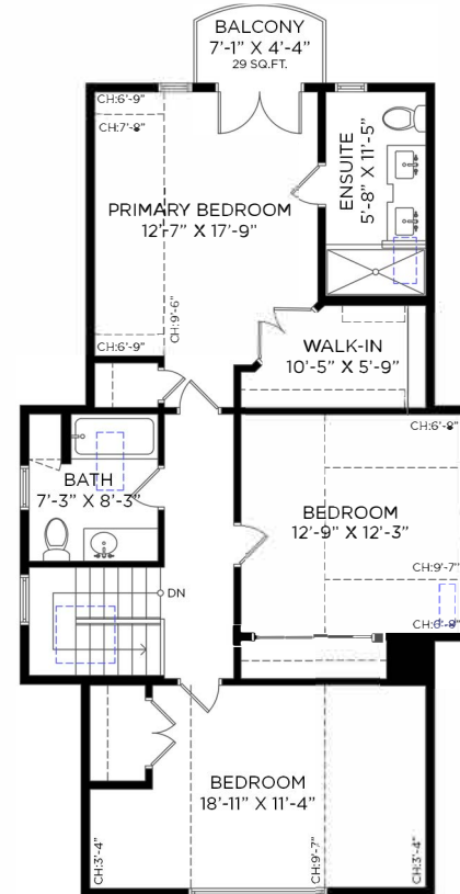
UPPER FLOOR - 949 SQ.FT. CEILING HEIGHT: 3'-4" TO 9'-7"
