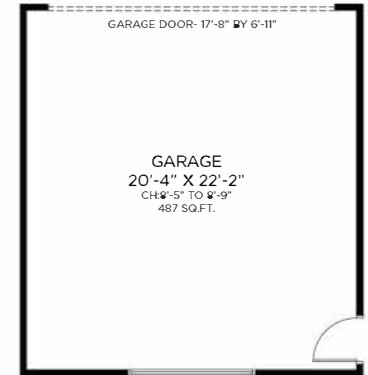
GARAGE - 487 SQ.FT. CEILING HEIGHT: 8'-5" TO 8'-9"
