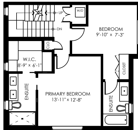
Upper Floor: 680 Sq.Ft. Ceiling Height: 8'-5"
