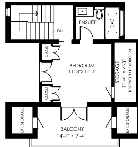
Top Floor: 344 Sq.Ft. Vaulted Ceiling Height: 9'-6"
