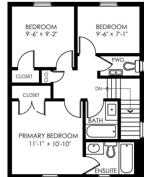
Upper Floor: 548 Sq.Ft. Ceiling Height: 10'-1"
