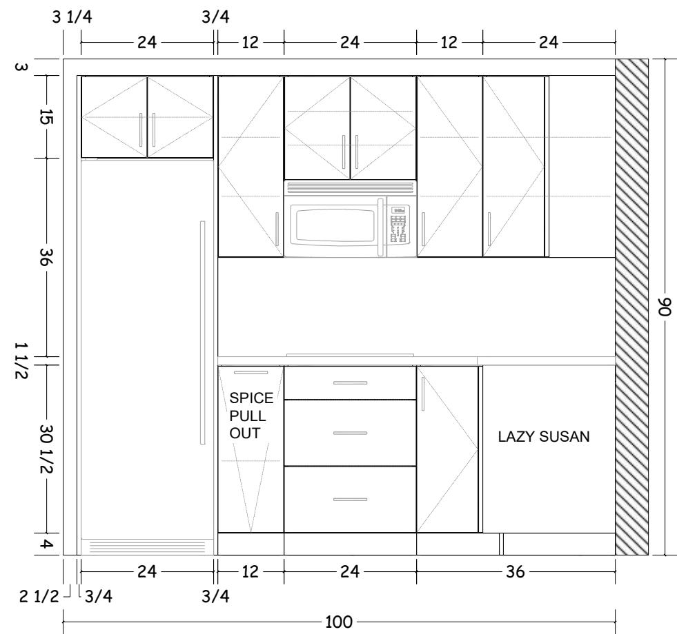
1 Kitchen Elevation A-1 Scale : 1/2" = 1'
