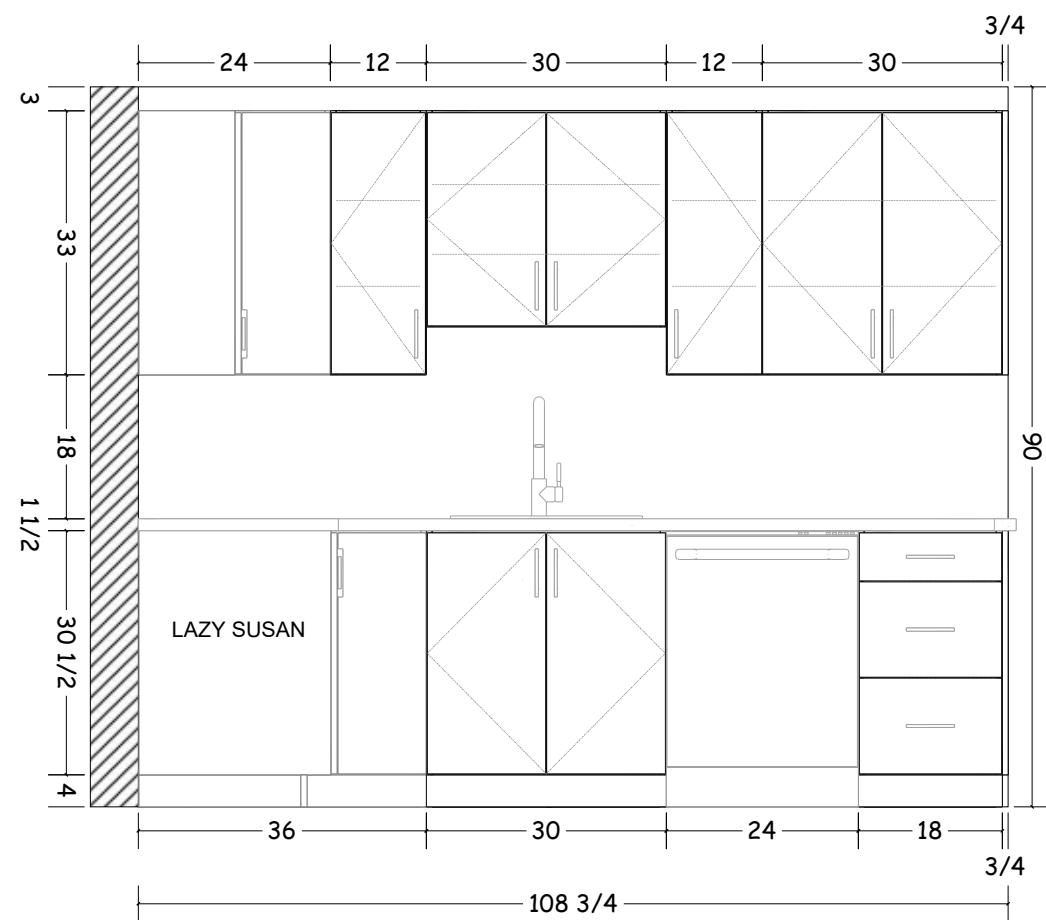
2 Kitchen Elevation A-1 Scale : 1/2" = 1'
