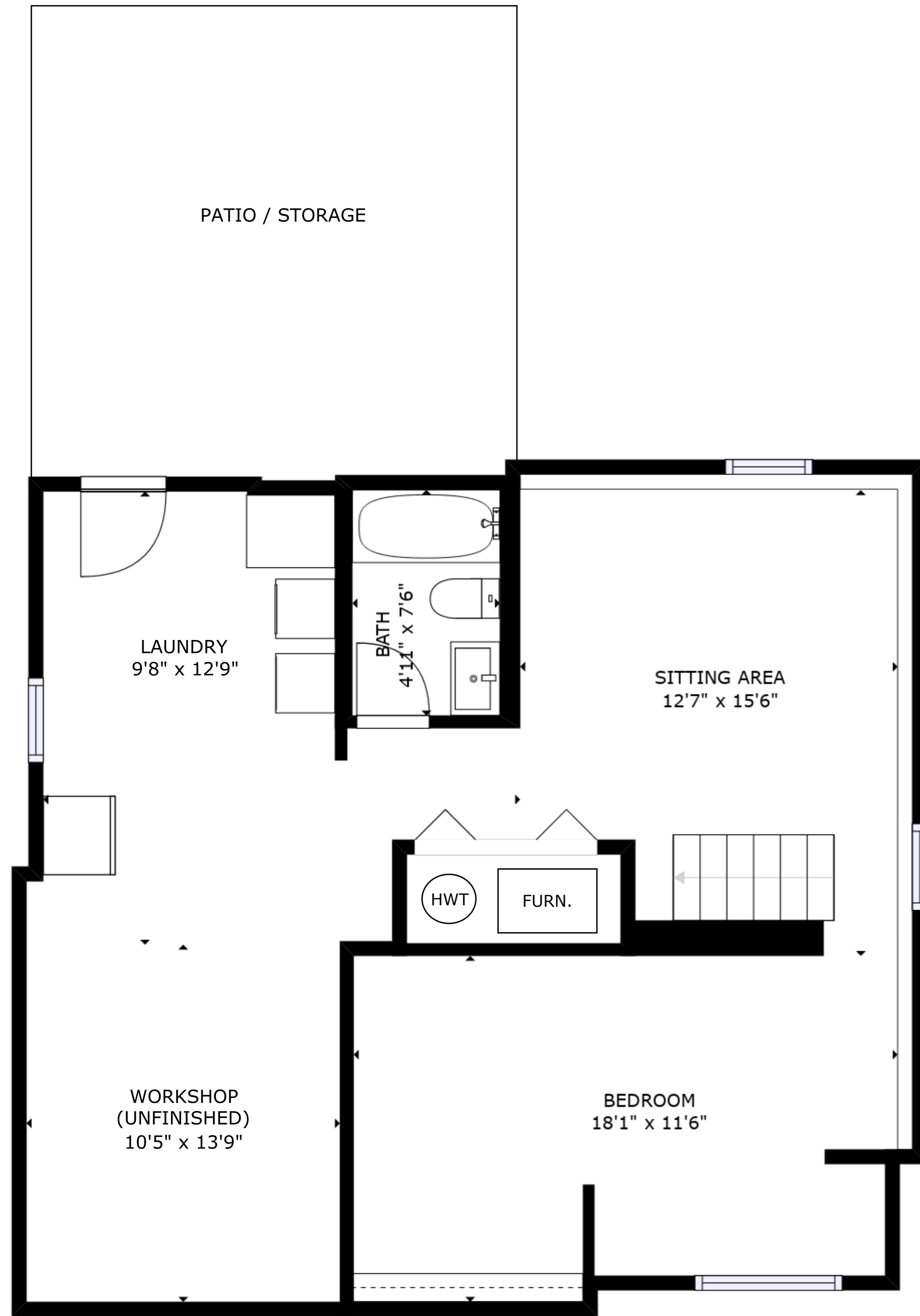
FLOOR 1 CEILING HEIGHT 6'3"
