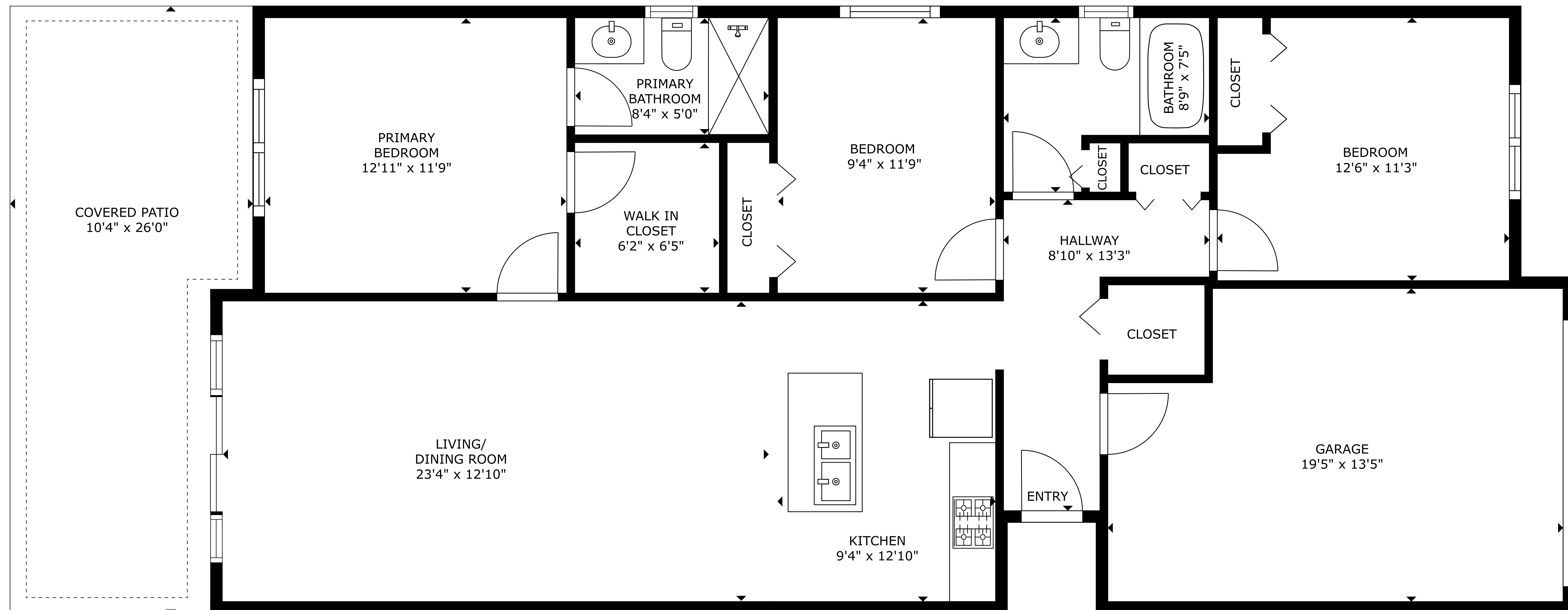
FLOOR PLAN
