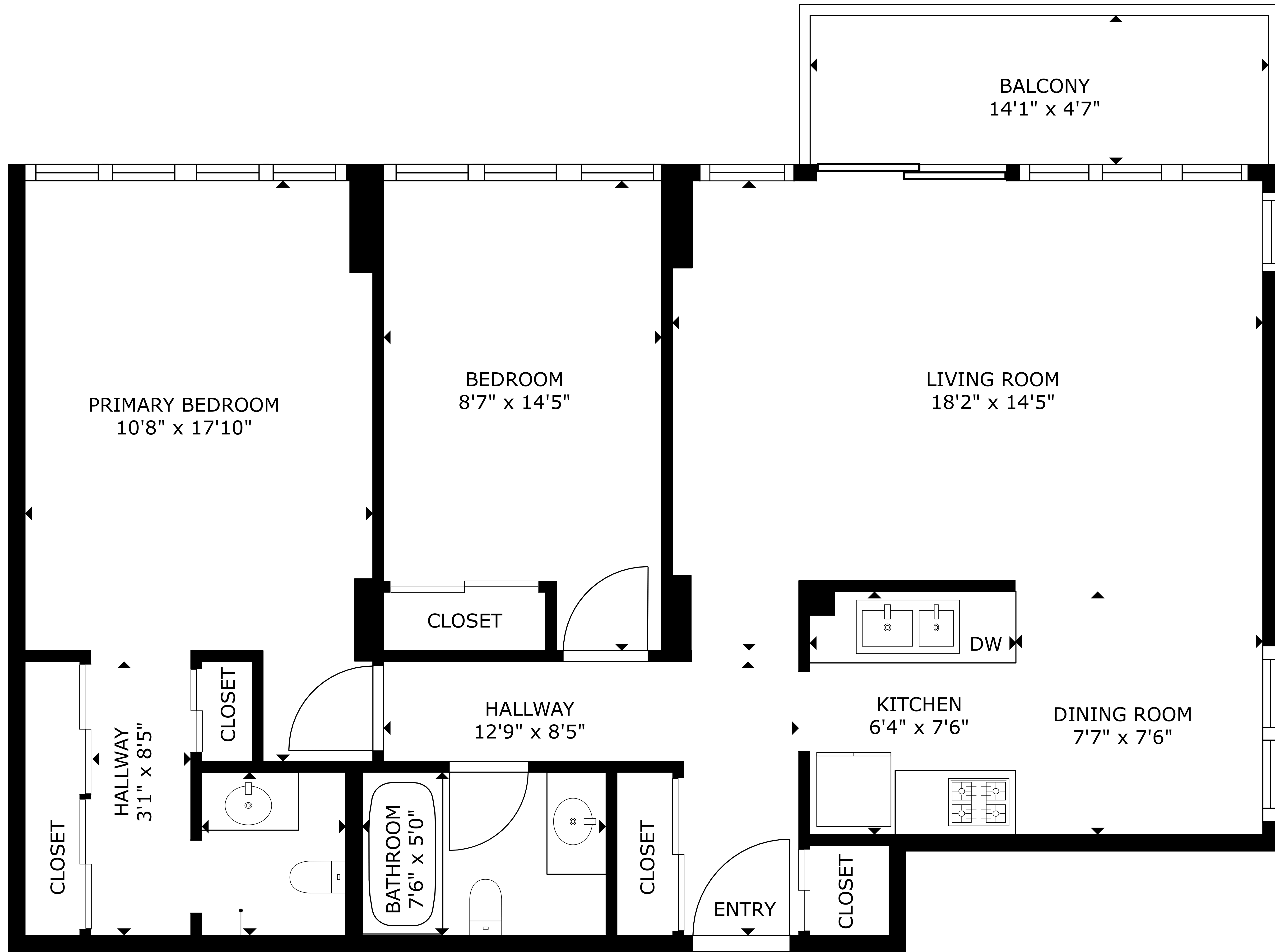
FLOOR PLAN PRIMARY BATHROOM 4'5" x 5'0"
