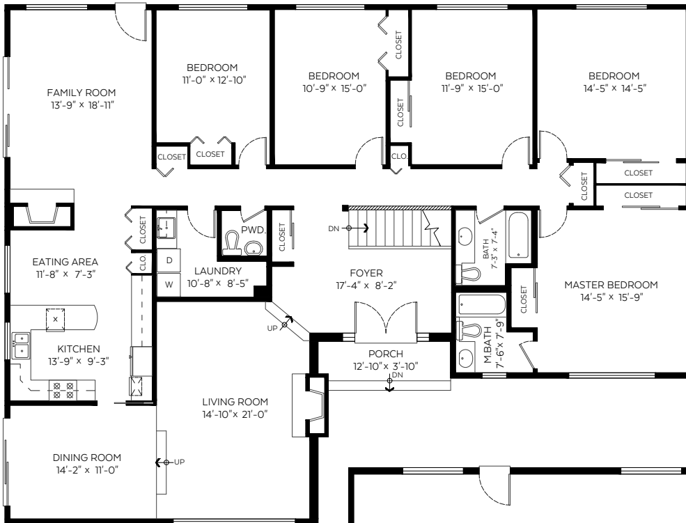
Main Floor Plan Floor Area: 2,768 sq.ft
