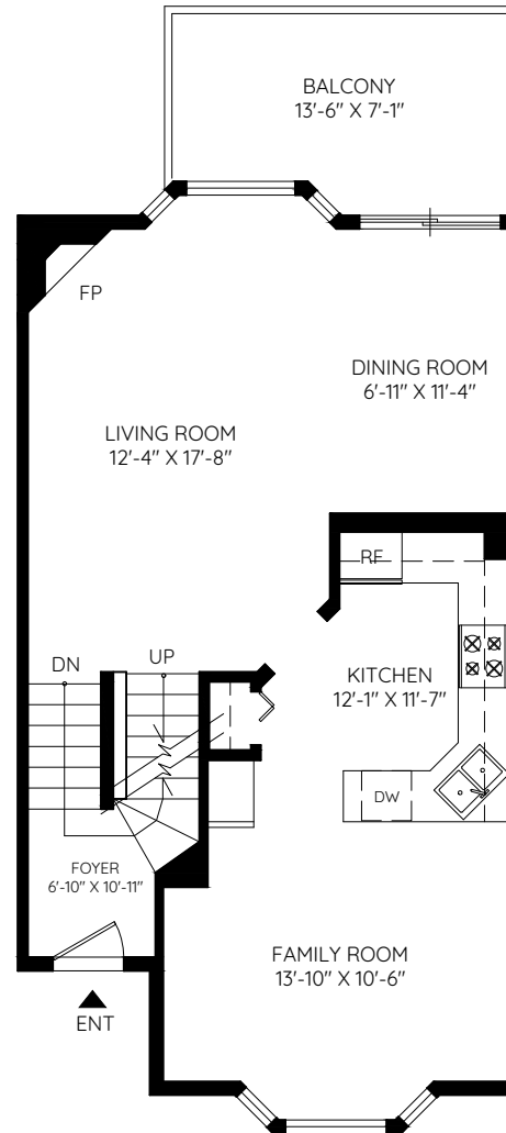
MAIN 698 SQ.FT. CEILING HEIGHT: 8'-0"
