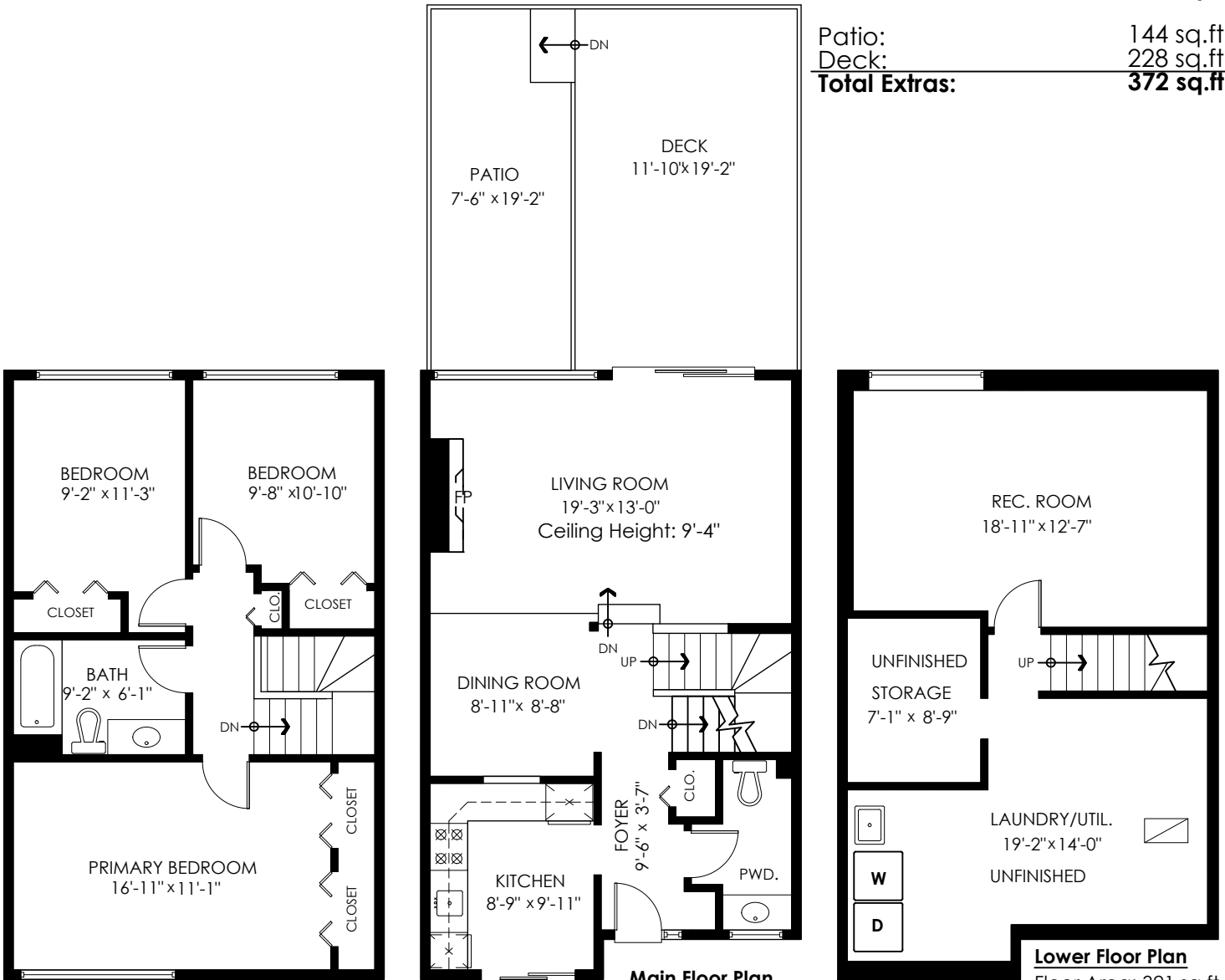
Upper Floor Plan Floor Area: 657 sq.ft. Ceiling Height: 8'
