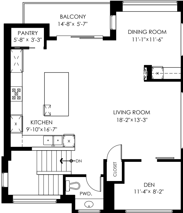
Upper Floor Plan Floor Area: 997 sq.ft. Ceiling Height: 9'
