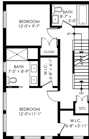
Upper Floor Plan
