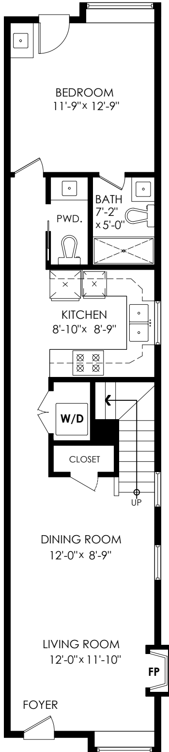
Main Floor Plan Floor Area: 747 sq.ft. Ceiling Height: 9'-0"
