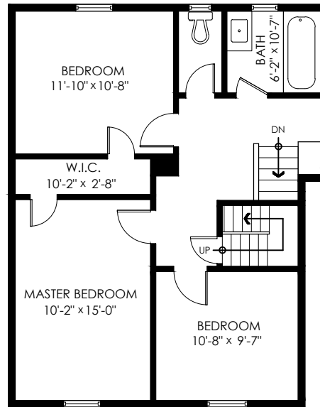
Upper Floor Plan Floor Area: 689 sq.ft. Ceiling Height: 7'-10"
