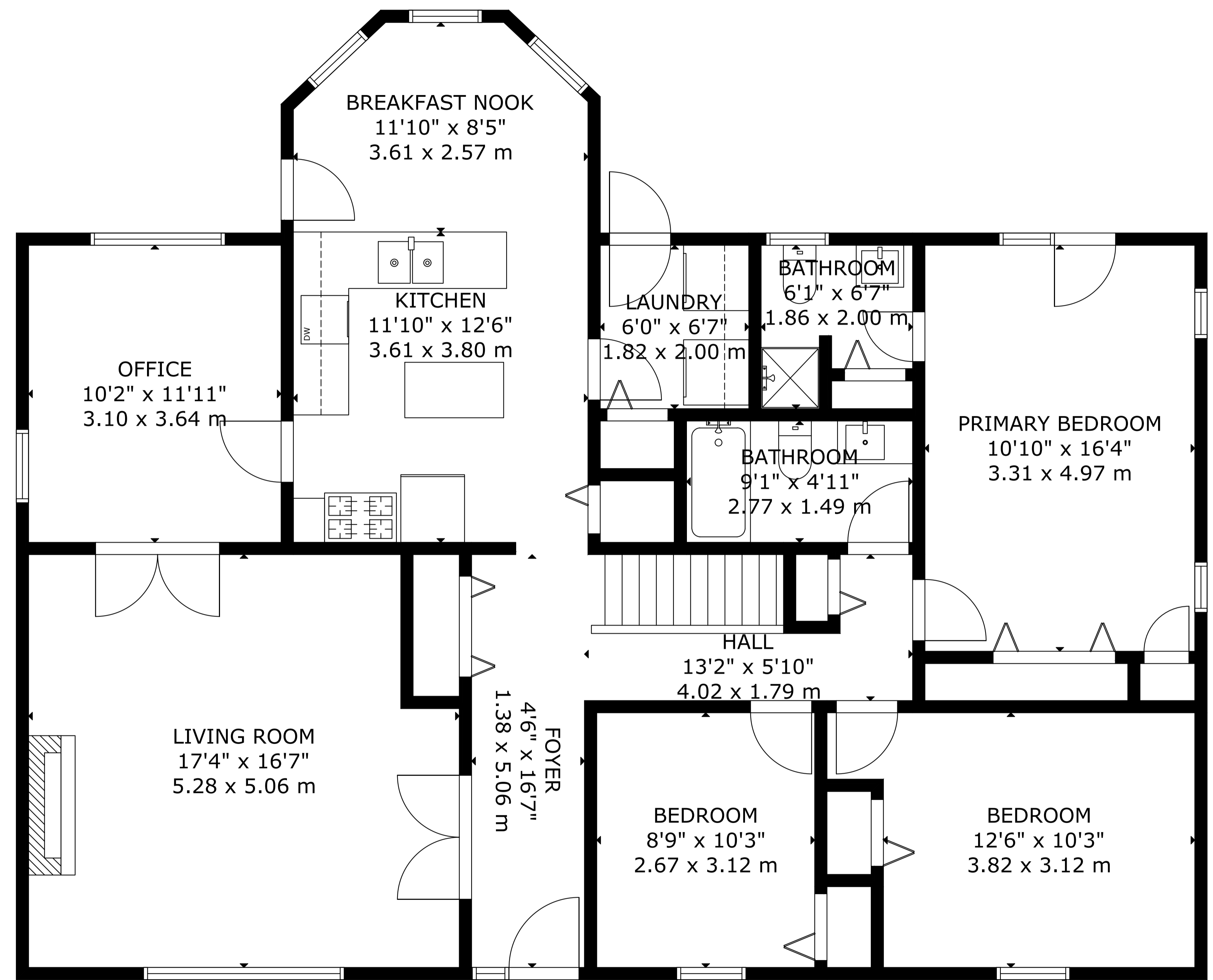
FIRST FLOOR
