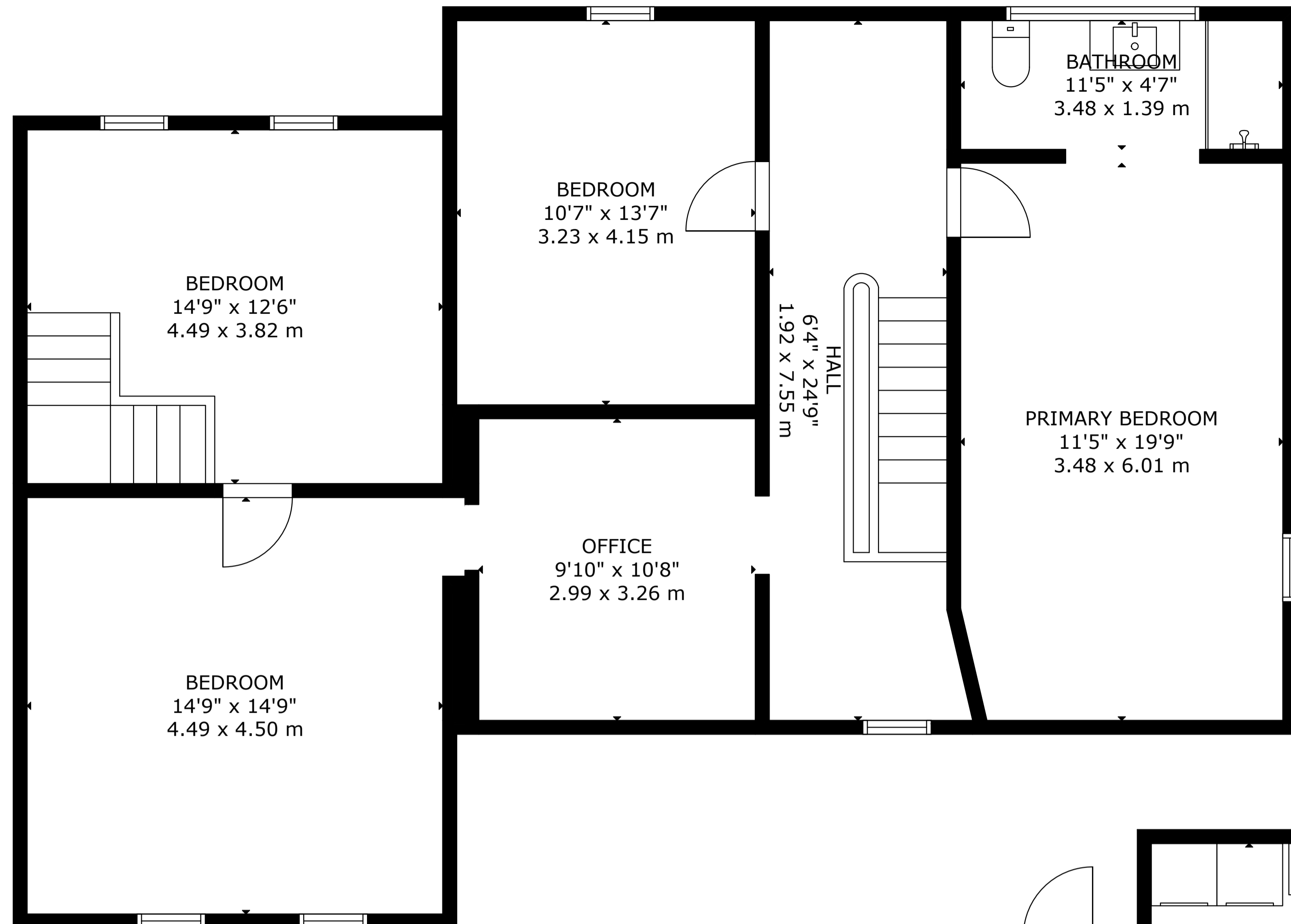
SECOND FLOOR
