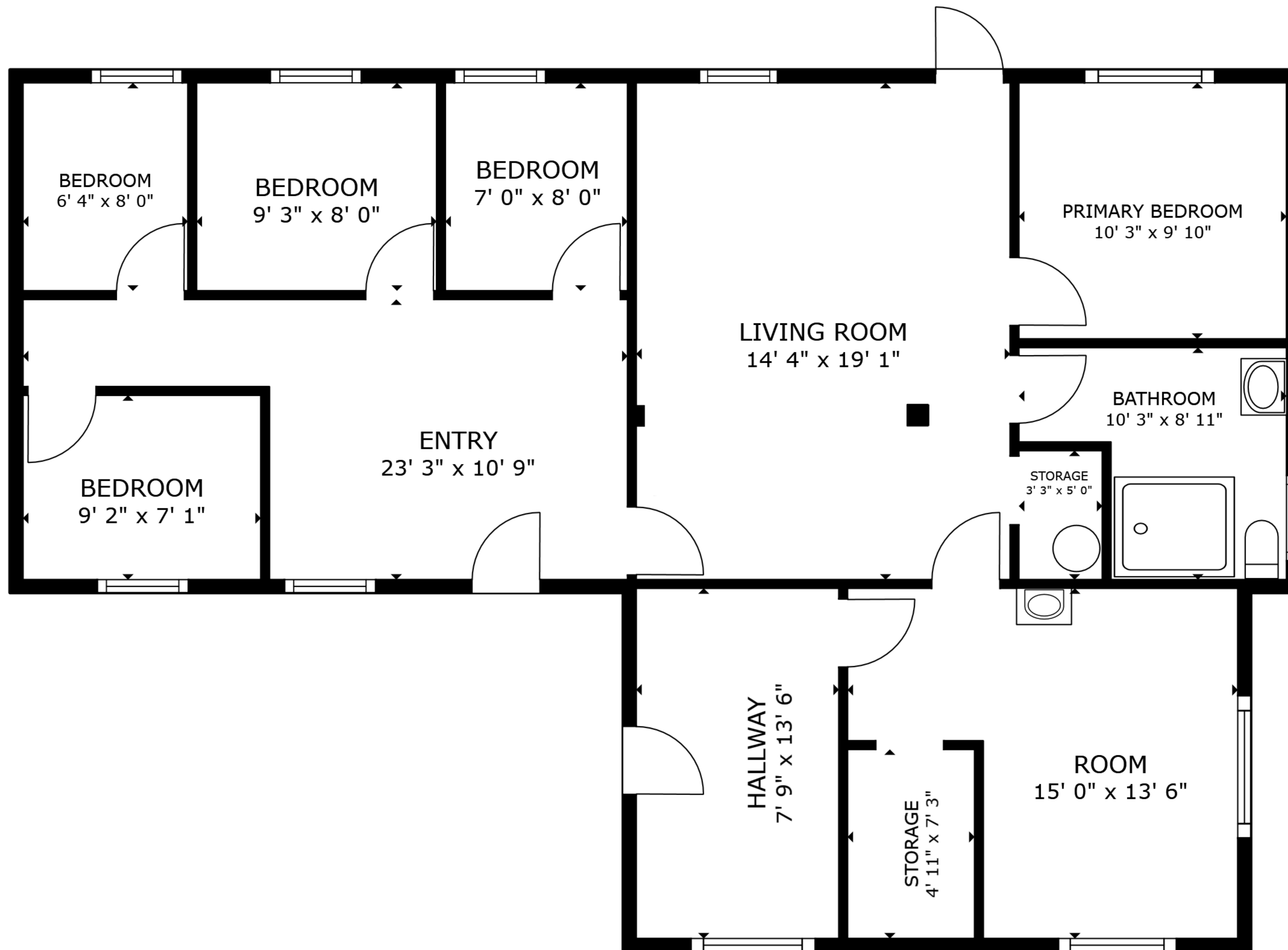
FLOOR PLAN
