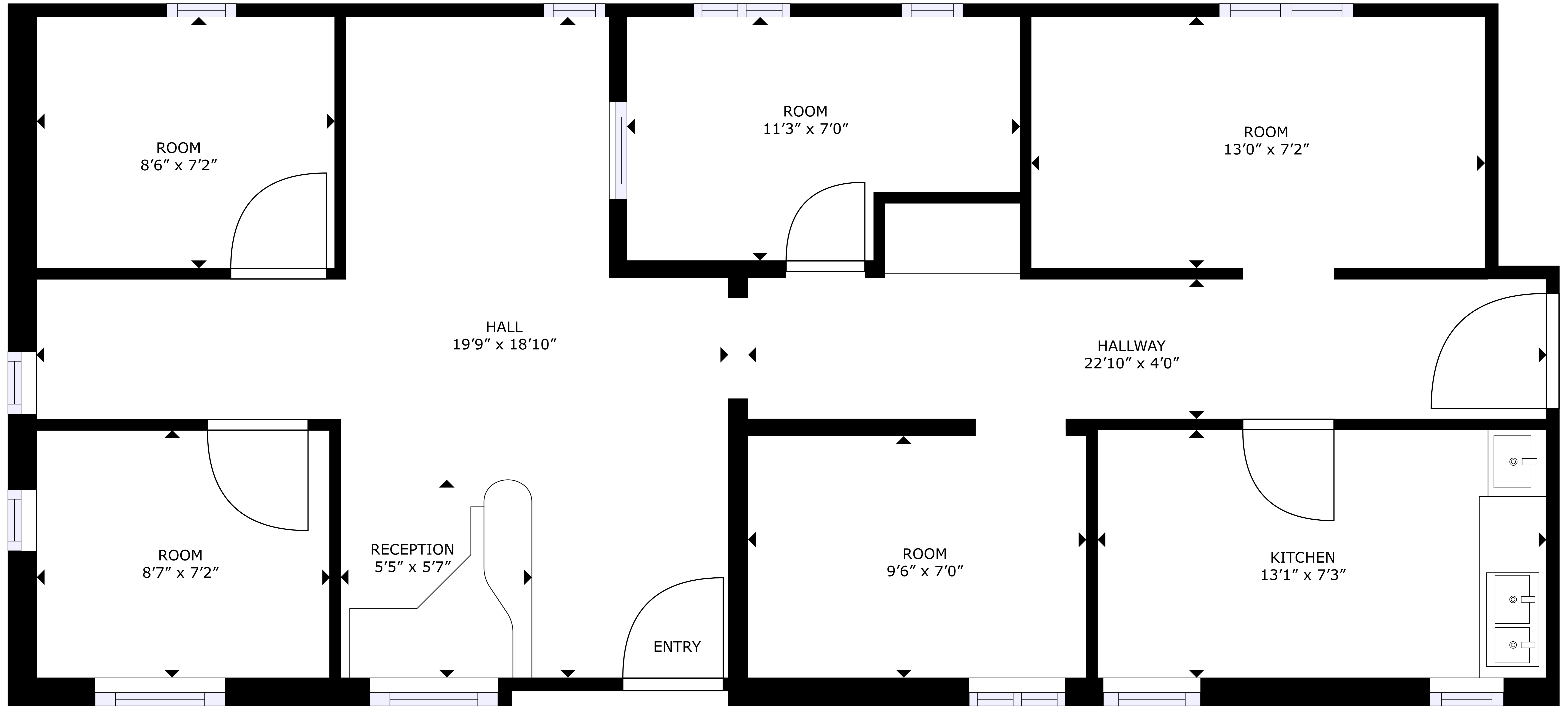
FLOOR PLAN
