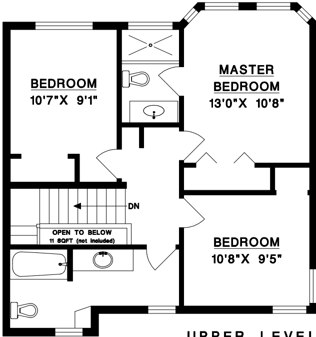
UPPER LEVEL
