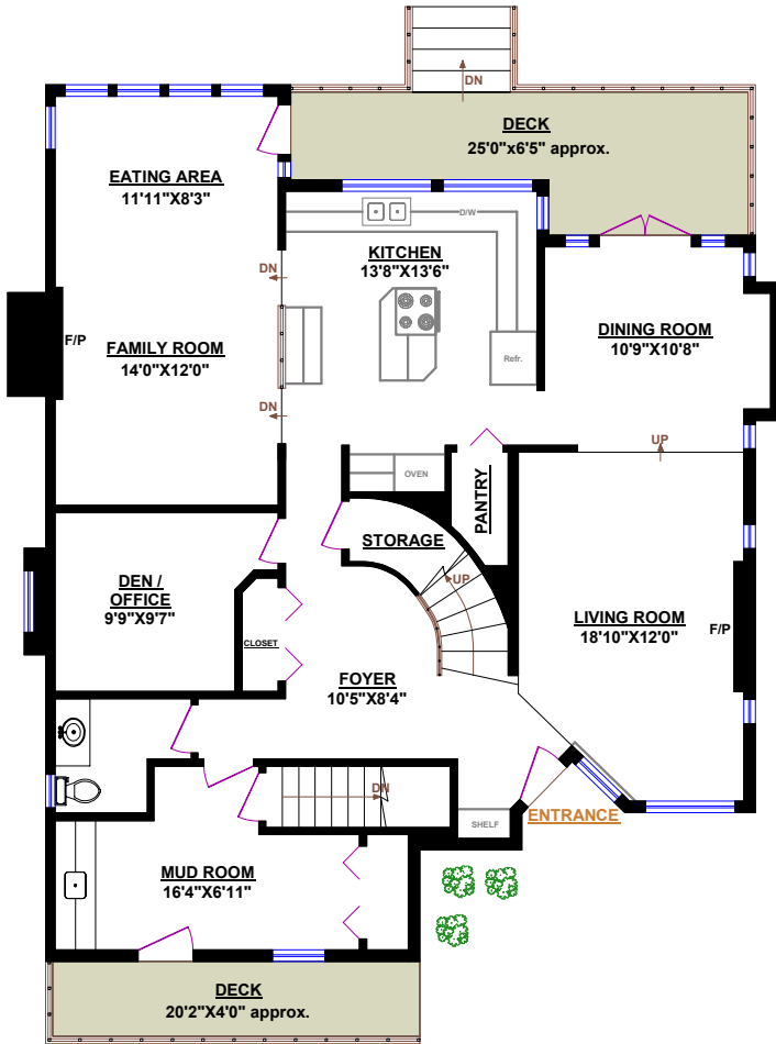
MAIN FLOOR
